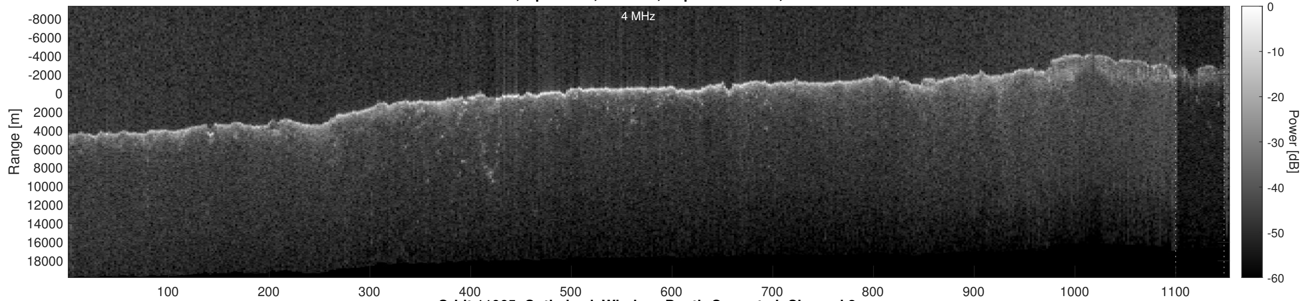
Orbit 11065, Optimized, Window, Depth-Corrected, Channel 2
