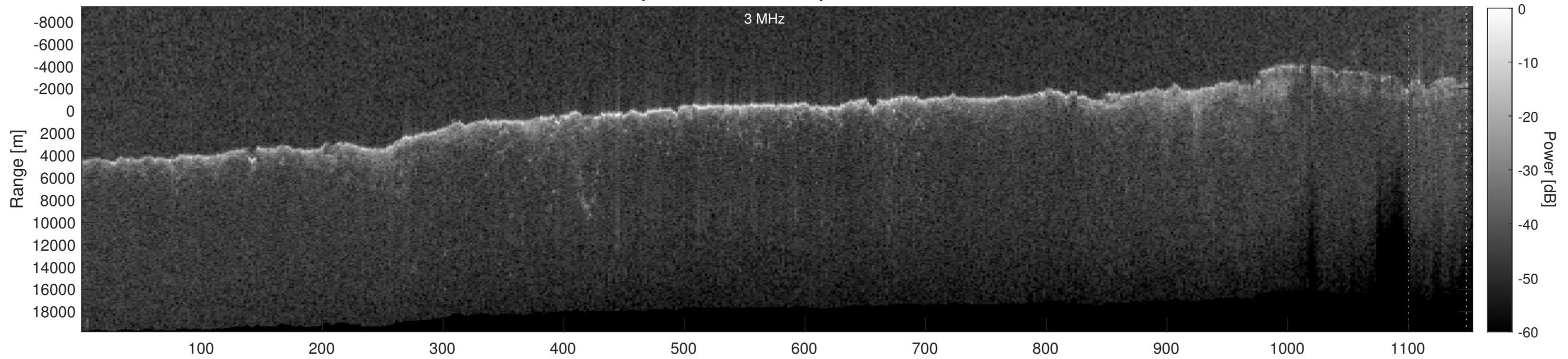
Orbit 11065, Depth-Corrected Cluttergram
