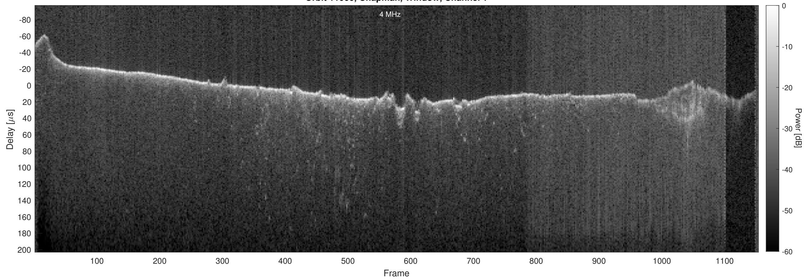
Orbit 11066, Chapman, Window, Channel 2
