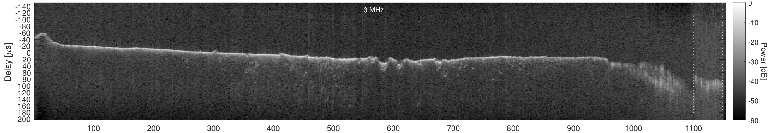
Orbit 11066, Window, Channel 2, Chapman
