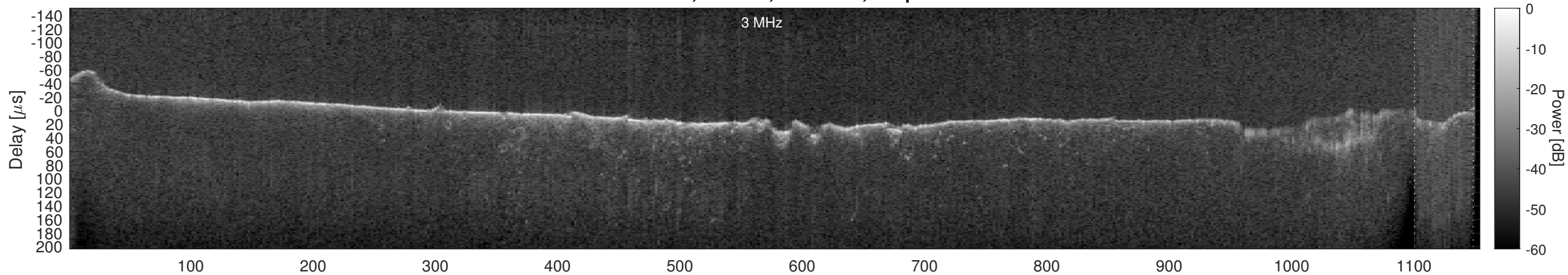
Orbit 11066, Window, Channel 2, Optimized
