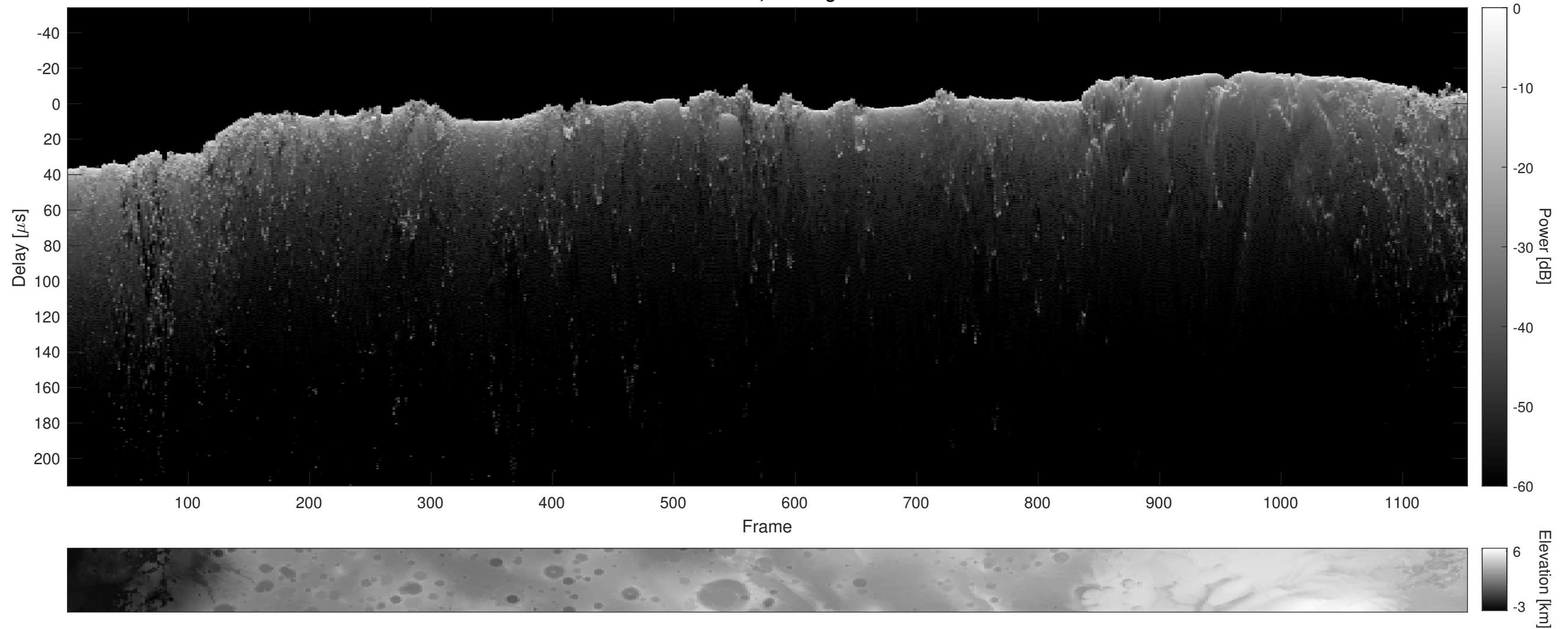
Orbit 11067, Cluttergram
