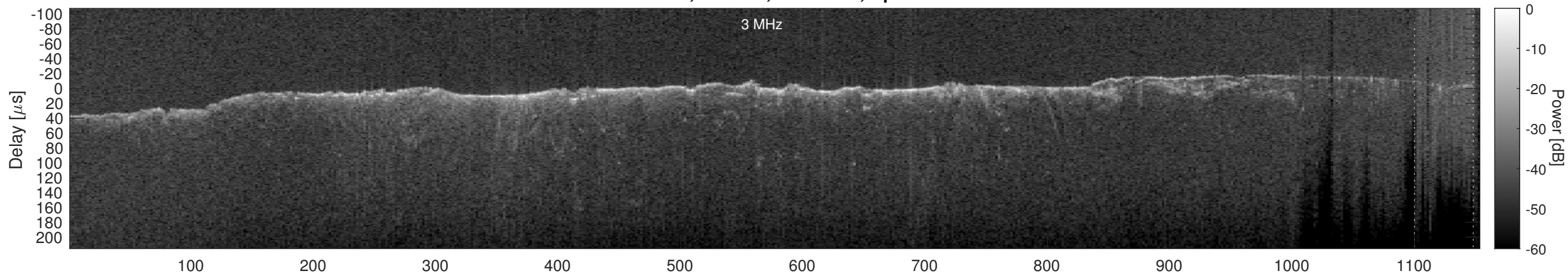
Orbit 11067, Cluttergram
