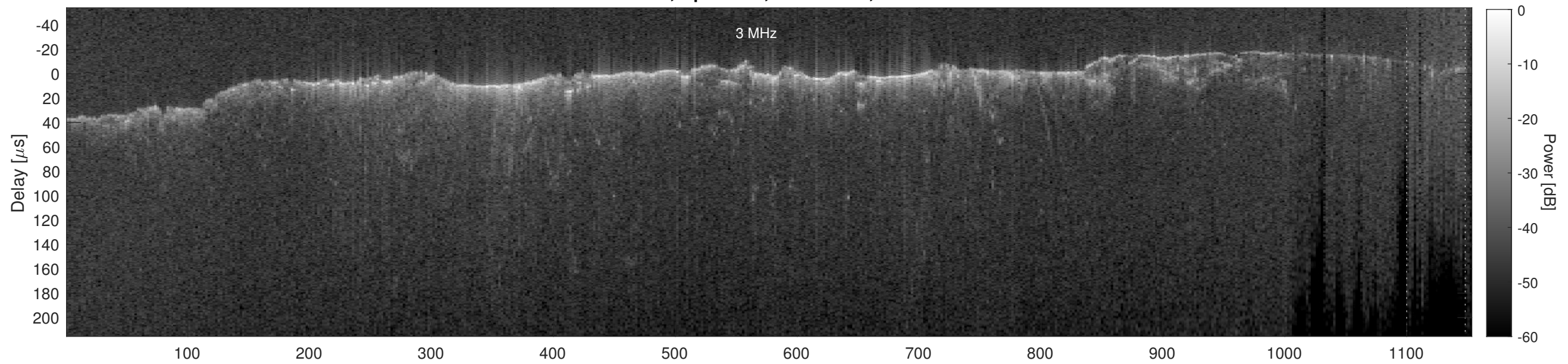
Orbit 11067, Cluttergram
