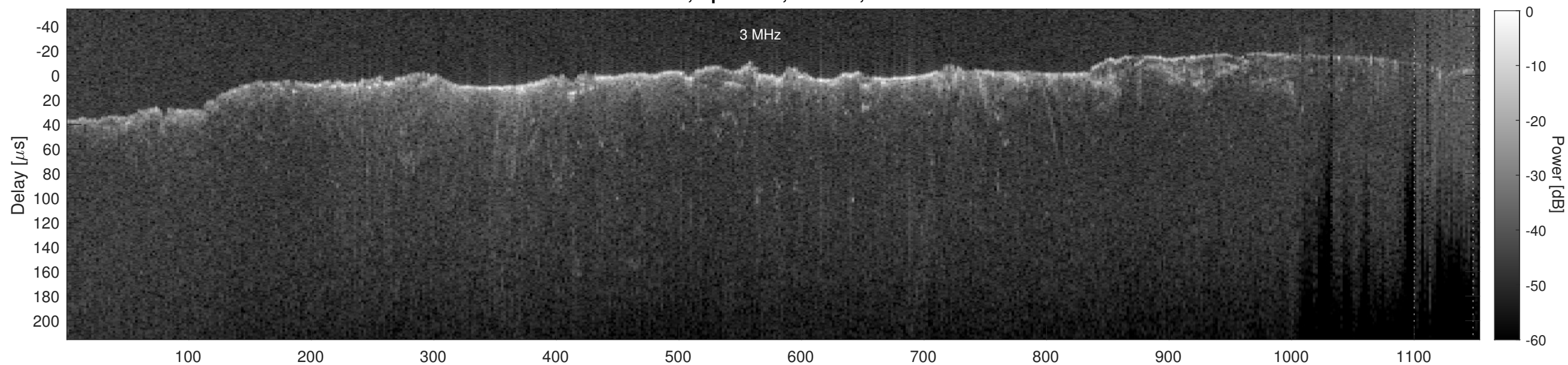
Orbit 11067, Cluttergram
