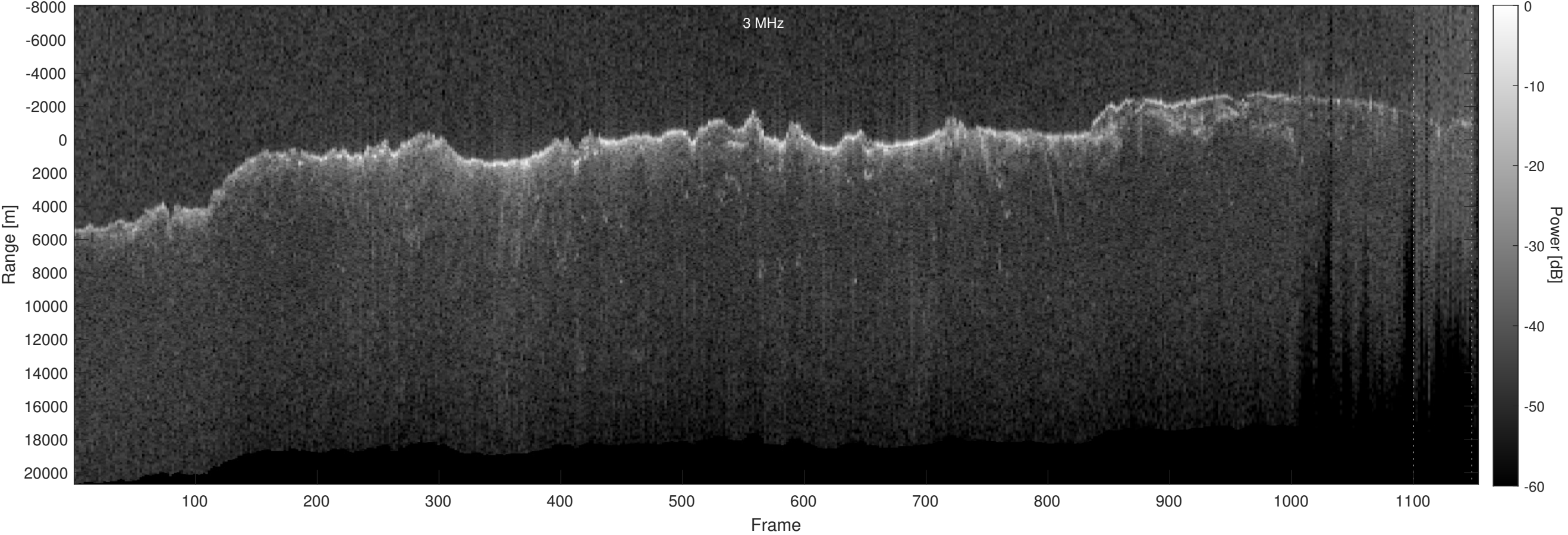
Orbit 11067, Optimized, Window, Depth-Corrected, Channel 2
