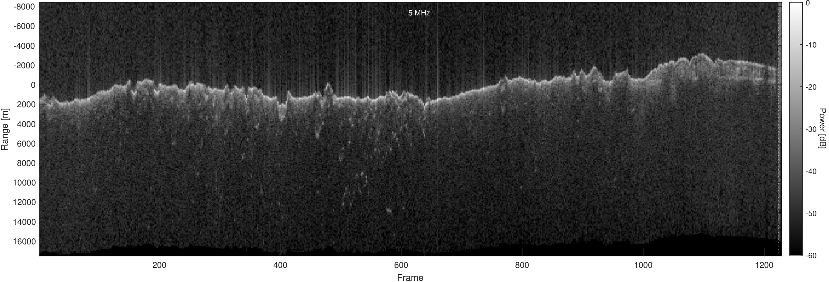
Orbit 11068, Optimized, Window, Depth-Corrected, Channel 2
