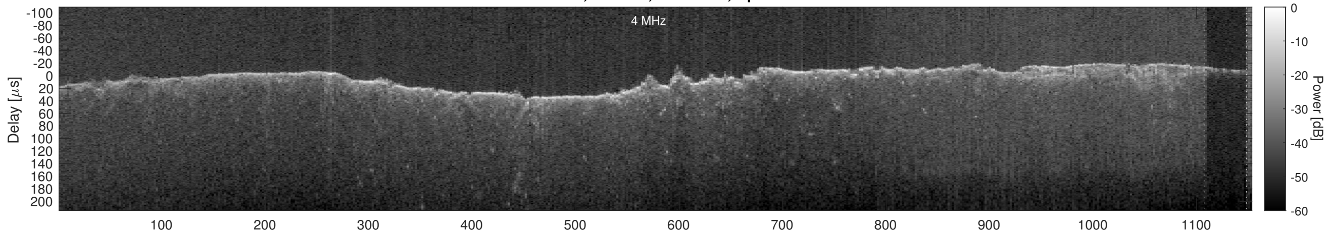
Orbit 11071, Cluttergram
