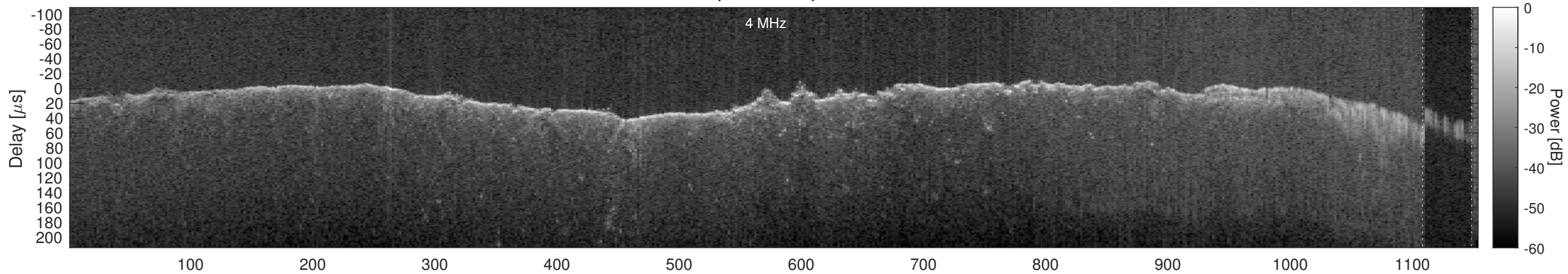
Orbit 11071, Window, Channel 1, Chapman
