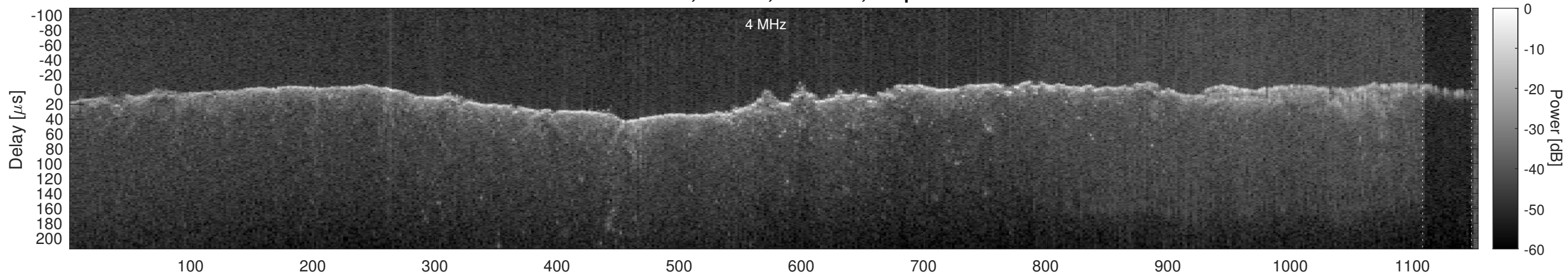
Orbit 11071, Window, Channel 1, Optimized
