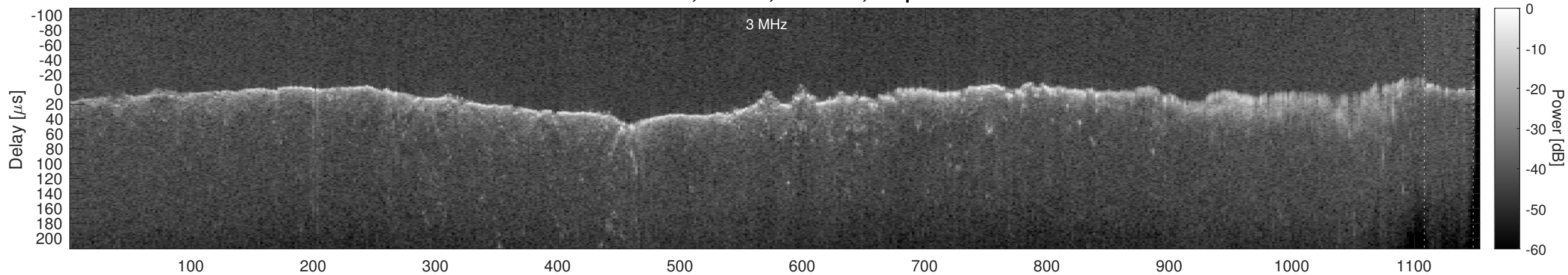
Orbit 11071, Window, Channel 2, Optimized
