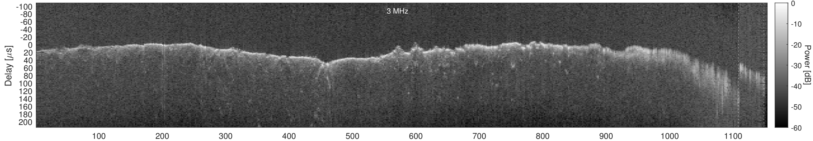
Orbit 11071, Window, Channel 2, Chapman
