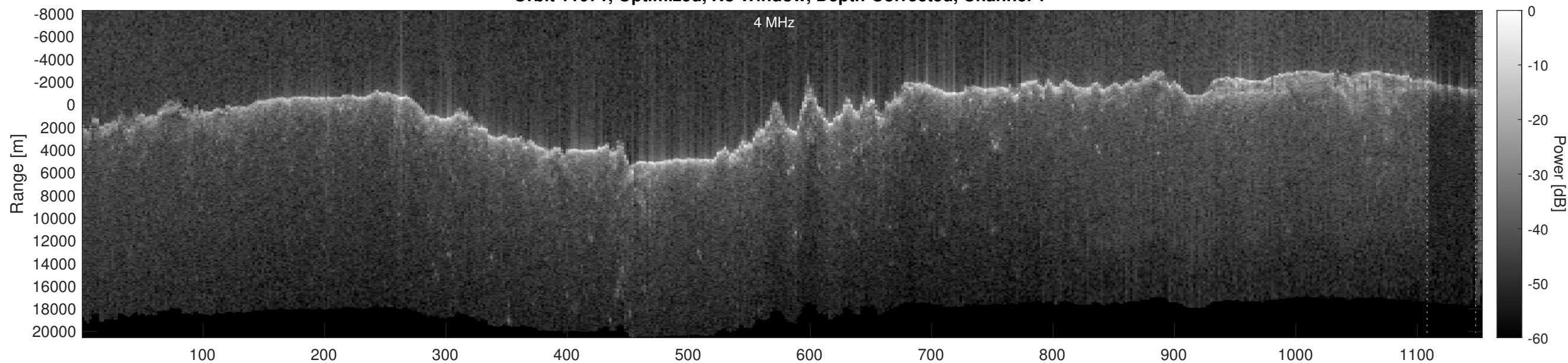
Orbit 11071, Optimized, No Window, Depth-Corrected, Channel 2
