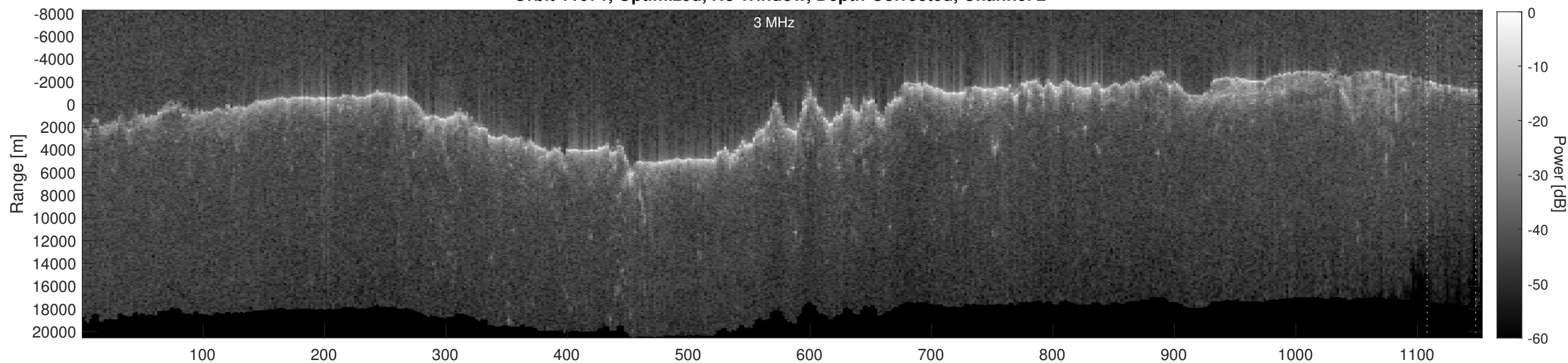
Orbit 11071, Depth-Corrected Cluttergram
