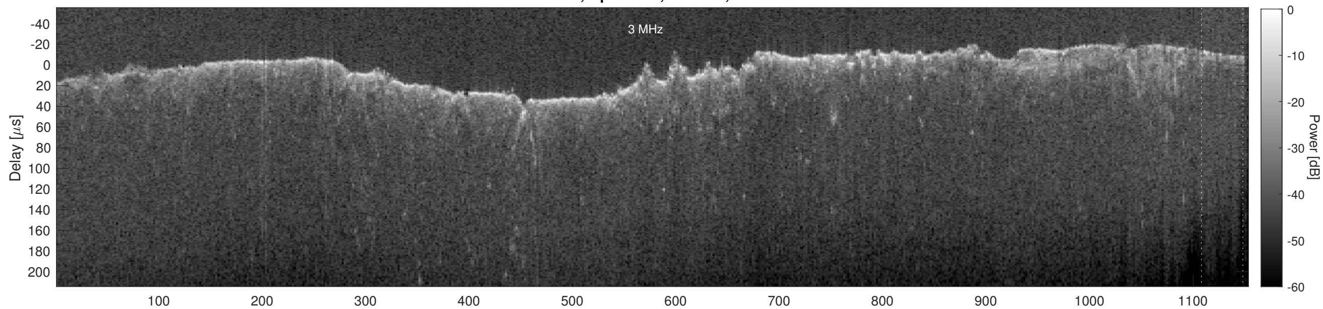
Orbit 11071, Cluttergram
