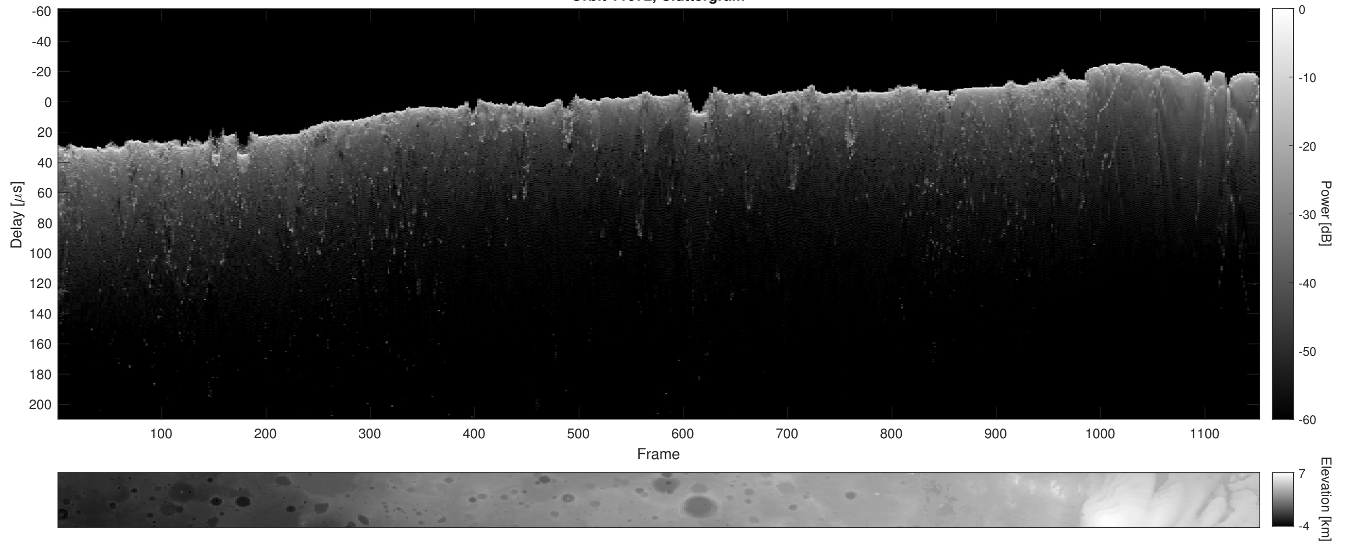
Orbit 11072, Cluttergram
