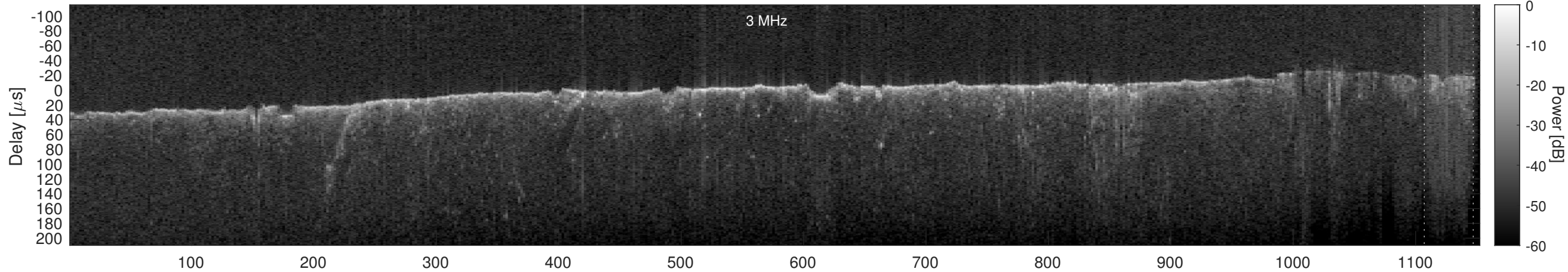
Orbit 11072, Cluttergram
