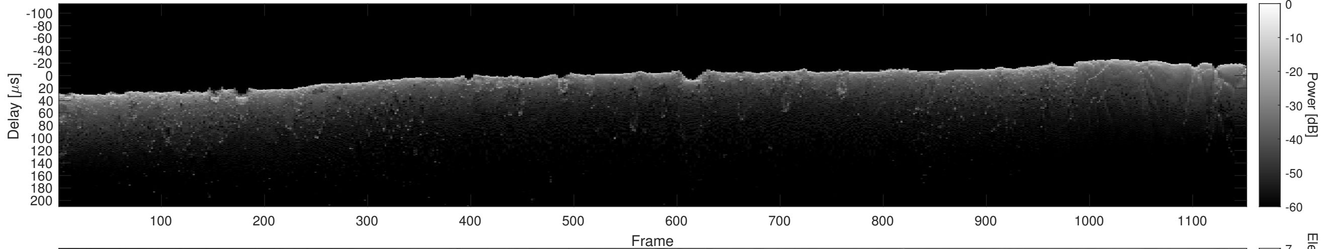
Orbit 11072, Cluttergram
