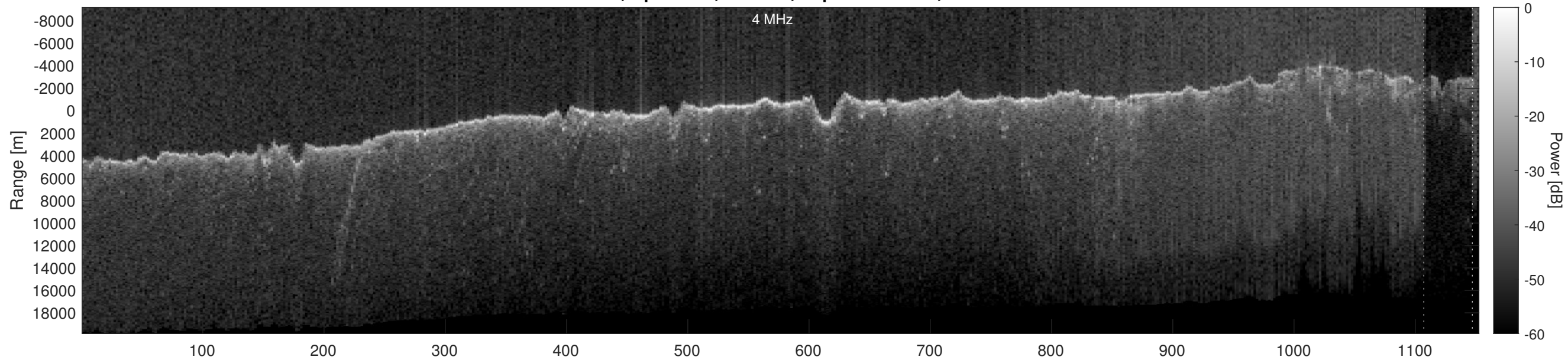
Orbit 11072, Optimized, Window, Depth-Corrected, Channel 2
