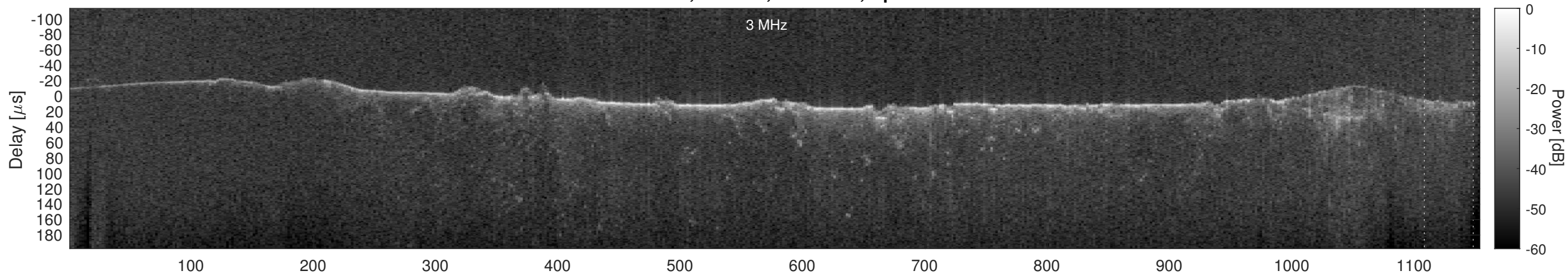
Orbit 11073, Cluttergram
