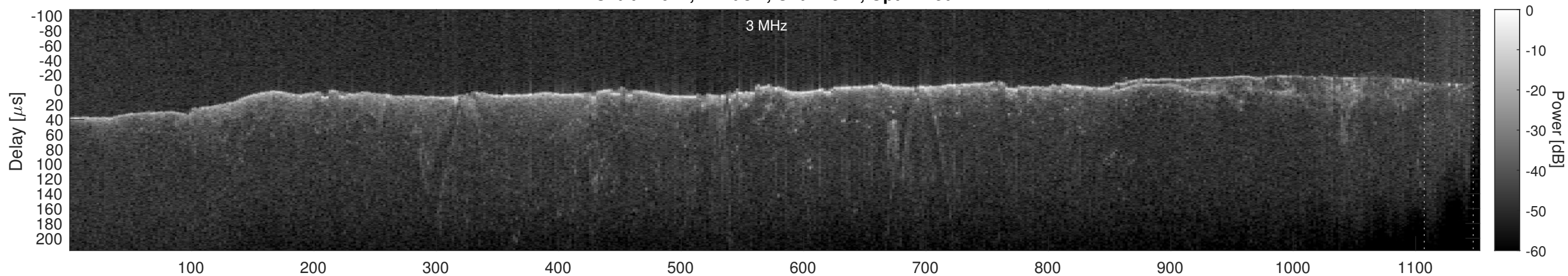
Orbit 11074, Cluttergram
