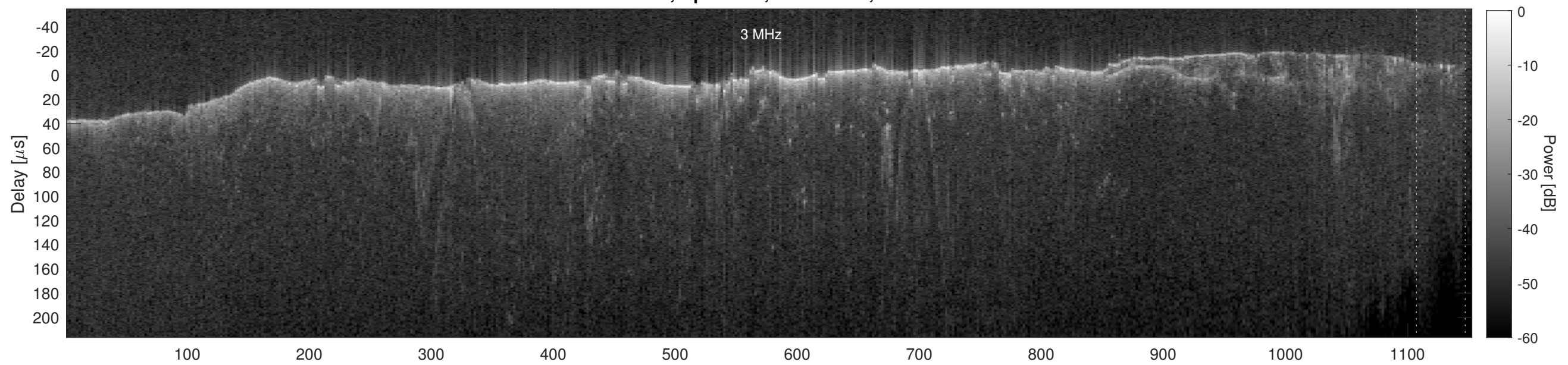
Orbit 11074, Cluttergram
