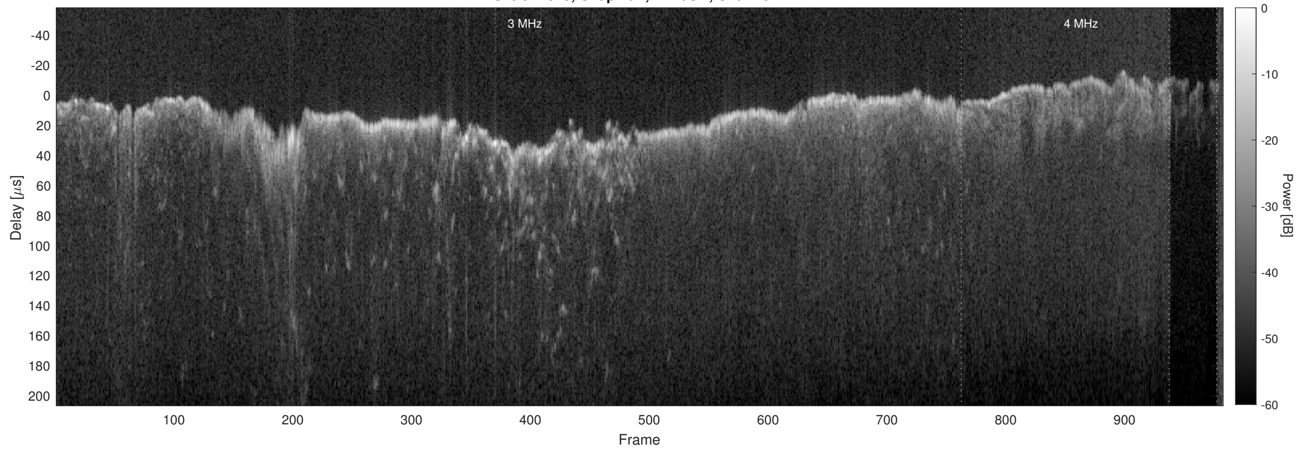
Orbit 11075, Chapman, Window, Channel 2
