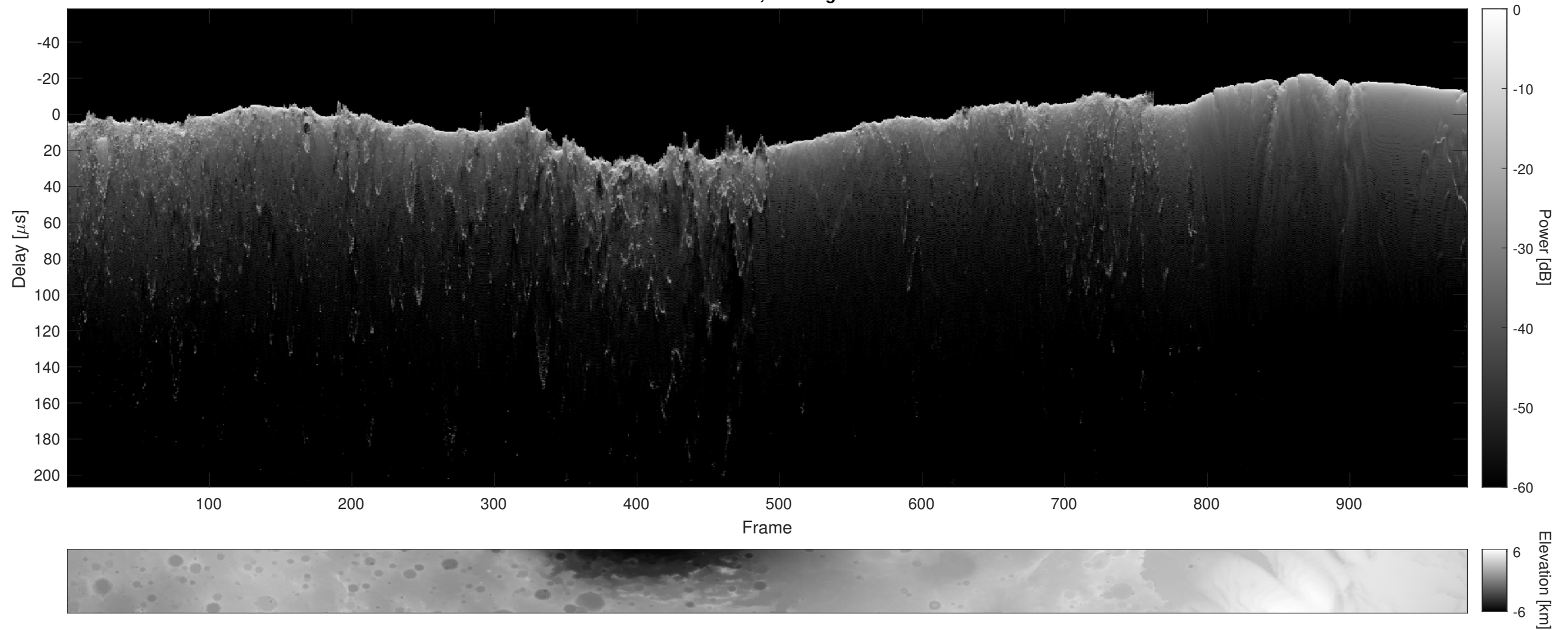
Orbit 11075, Cluttergram
