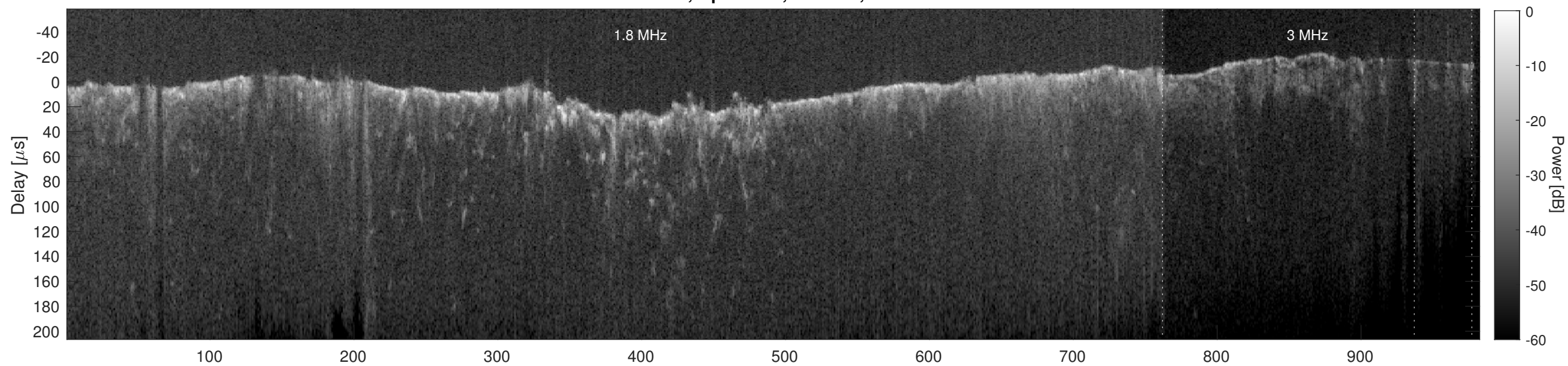
Orbit 11075, Cluttergram
