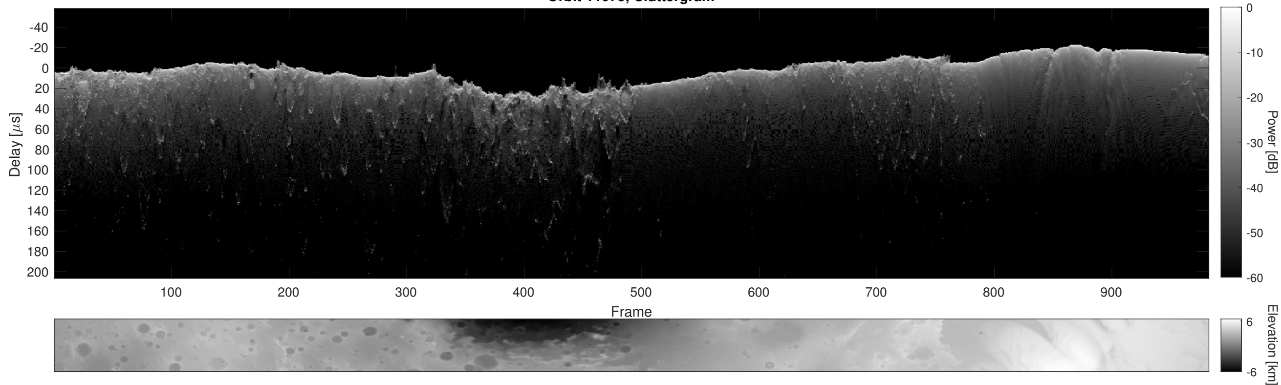
Orbit 11075, Cluttergram
