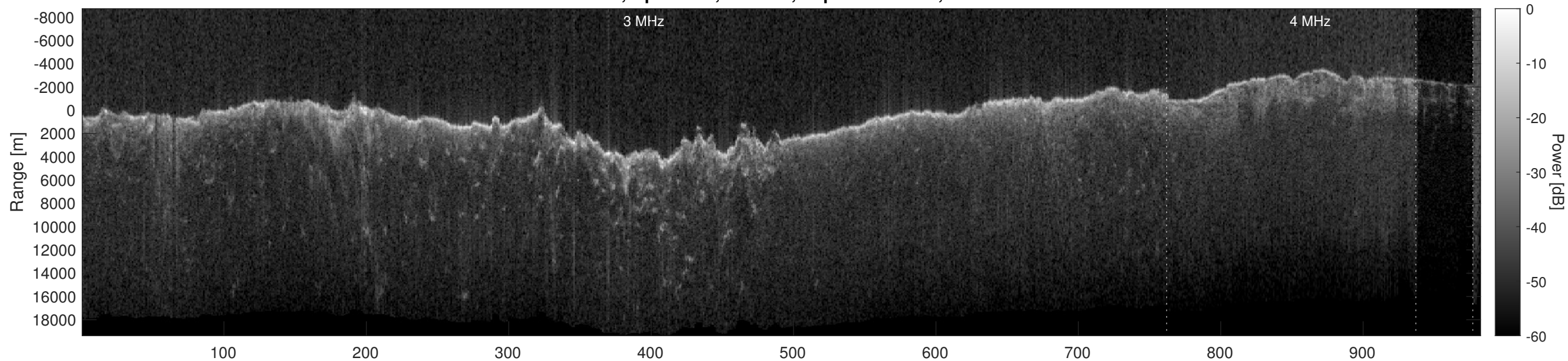
Orbit 11075, Optimized, Window, Depth-Corrected, Channel 2
