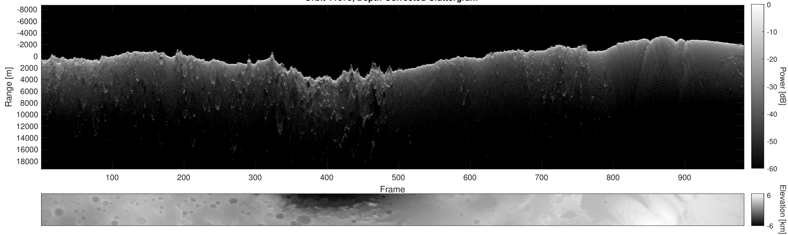
Orbit 11075, Depth-Corrected Cluttergram
