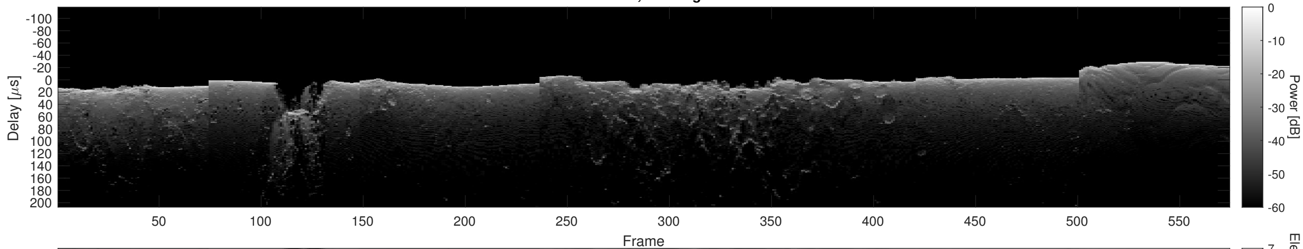
Orbit 11076, Cluttergram
