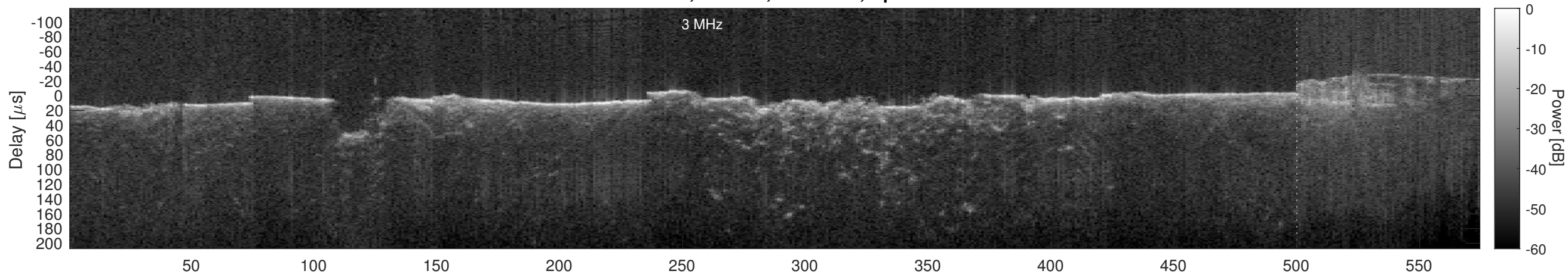
Orbit 11076, Cluttergram
