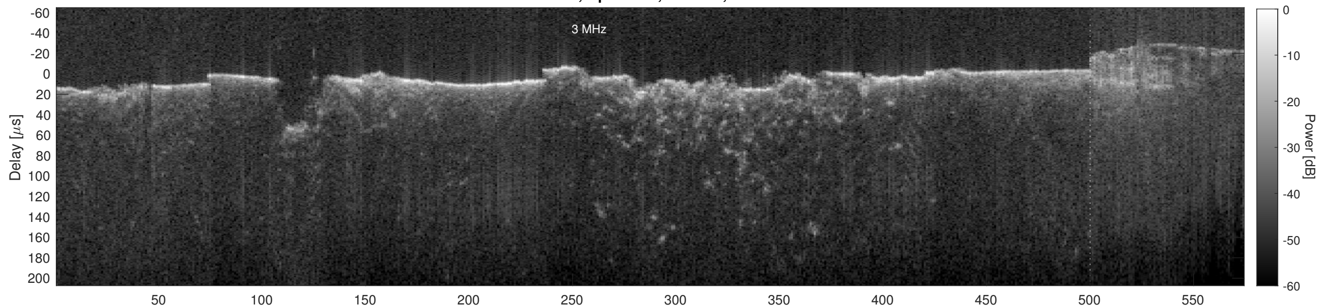
Orbit 11076, Cluttergram
