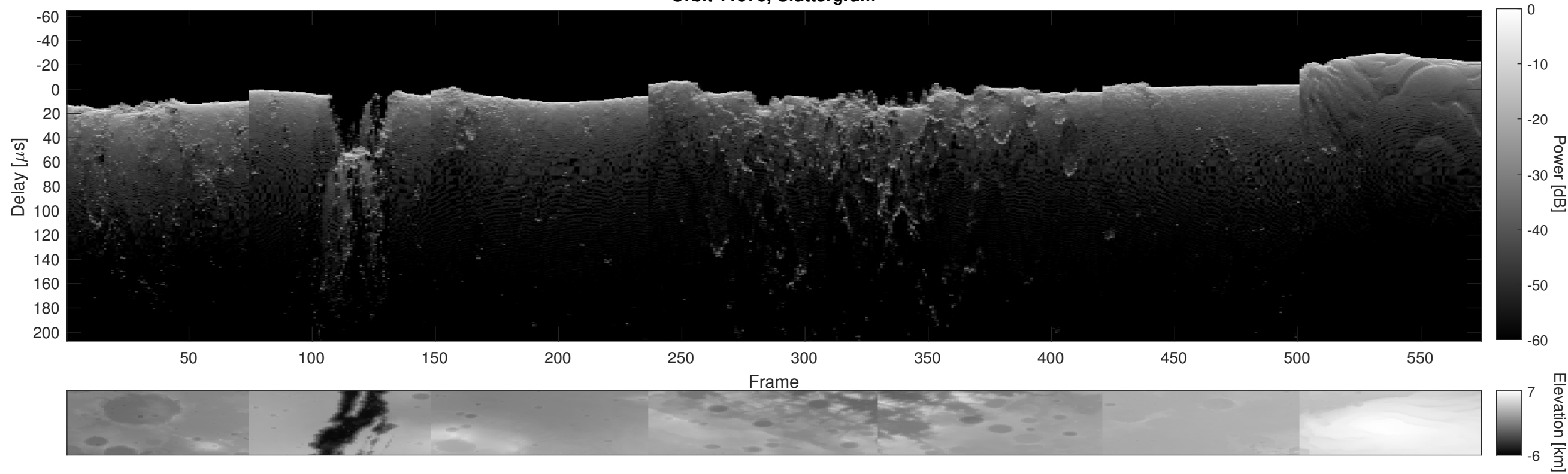
Orbit 11076, Cluttergram
