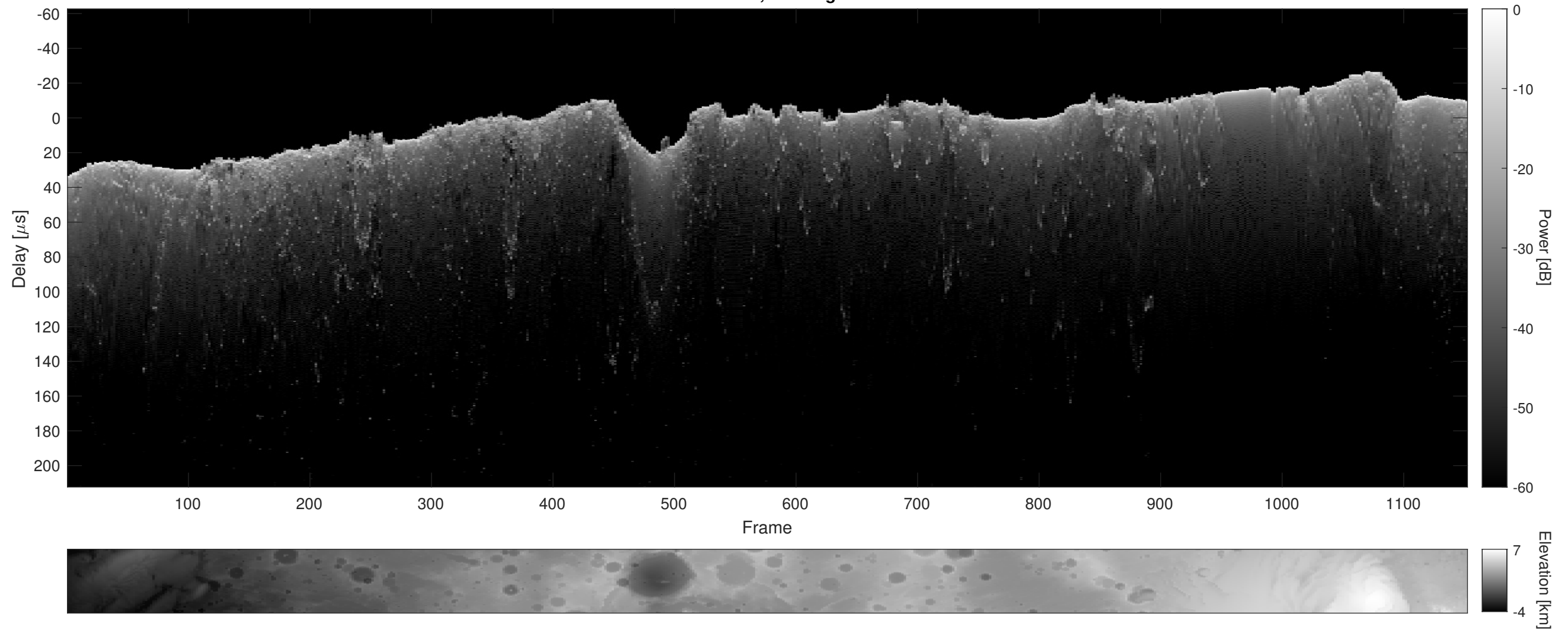
Orbit 11077, Cluttergram
