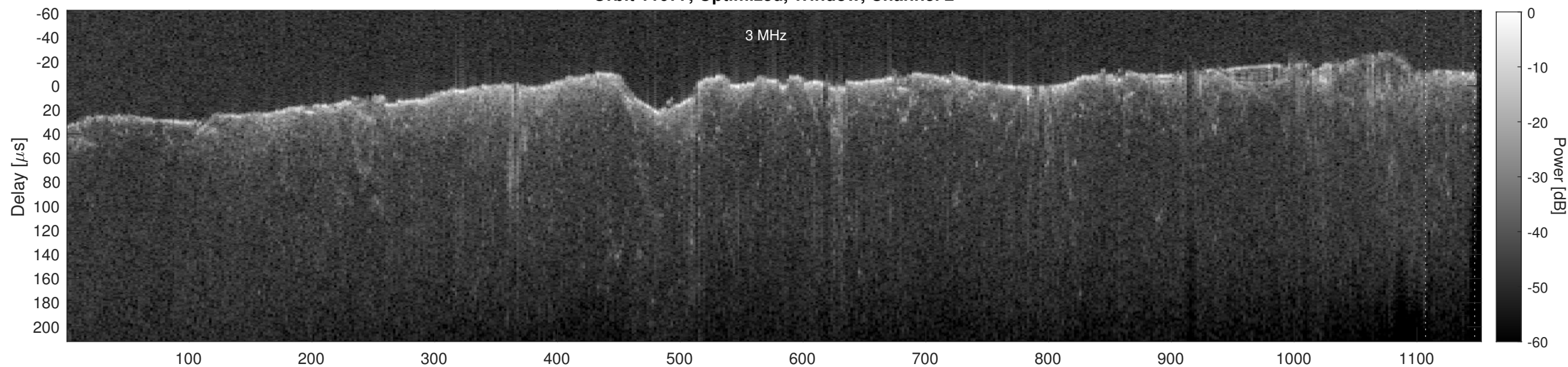
Orbit 11077, Cluttergram
