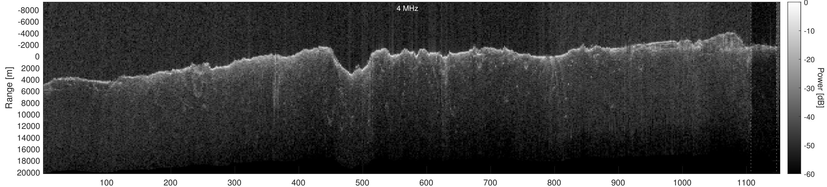
Orbit 11077, Optimized, Window, Depth-Corrected, Channel 2
