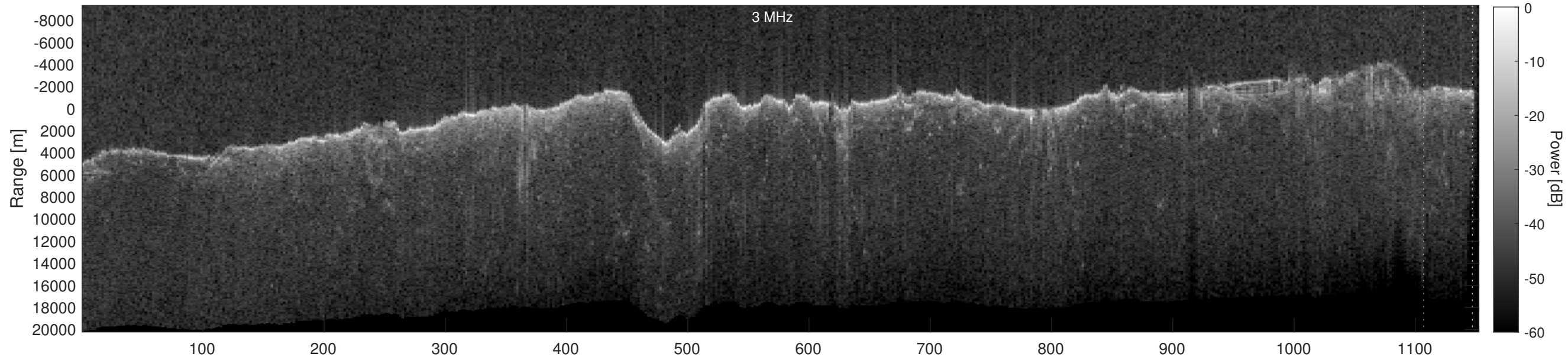
Orbit 11077, Depth-Corrected Cluttergram
