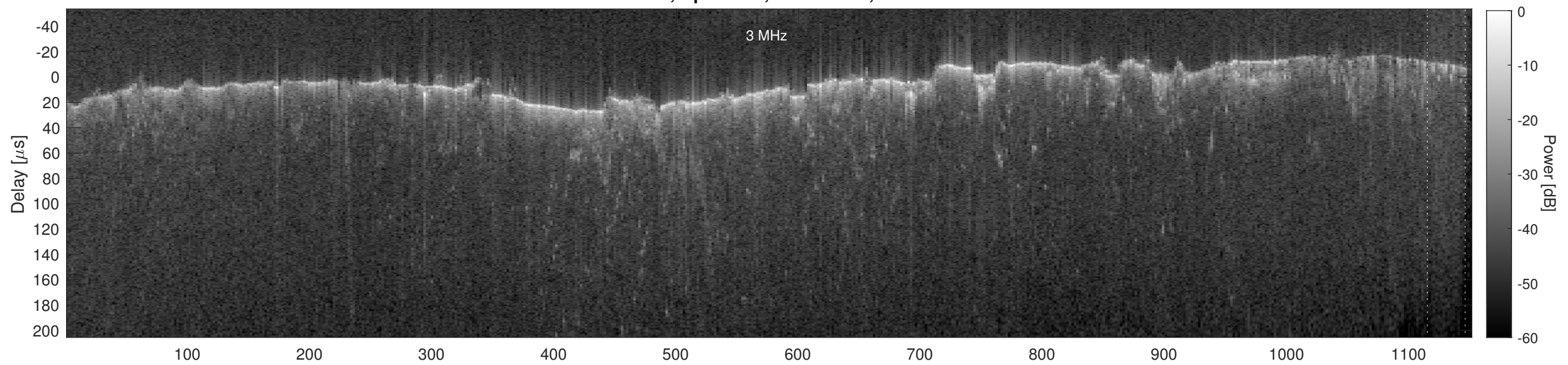
Orbit 11078, Cluttergram
