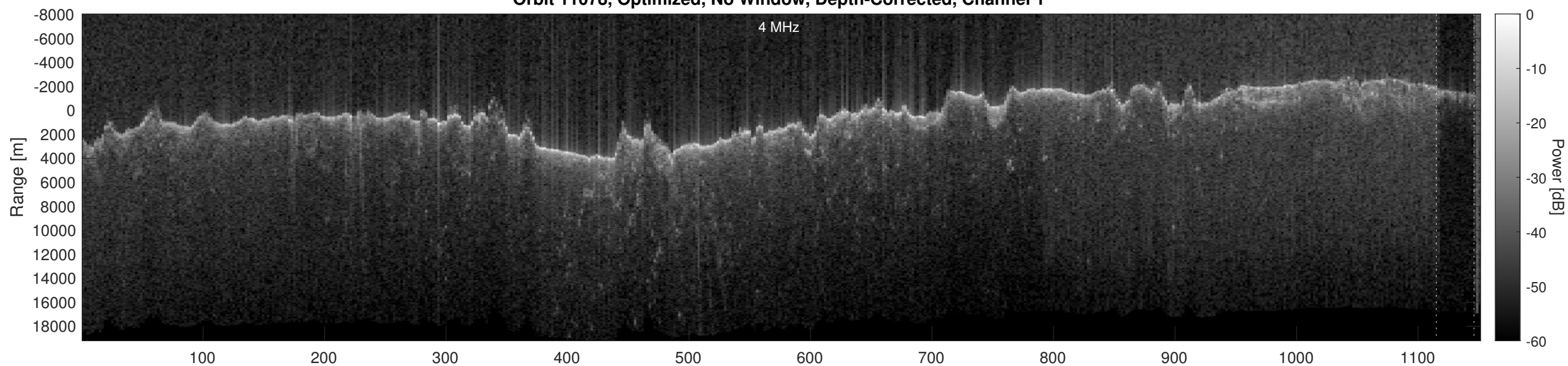
Orbit 11078, Optimized, No Window, Depth-Corrected, Channel 2
