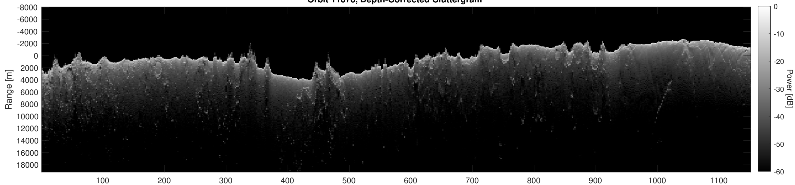
Orbit 11078, Depth-Corrected Cluttergram
