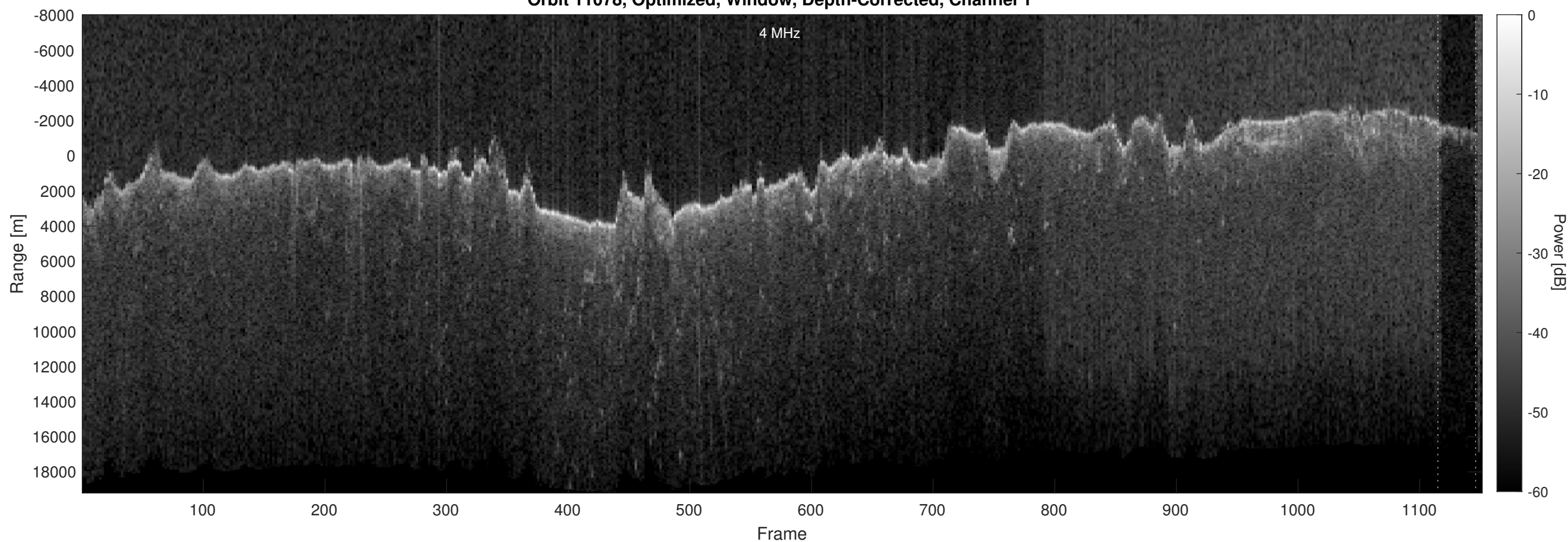
Orbit 11078, Optimized, Window, Depth-Corrected, Channel 2
