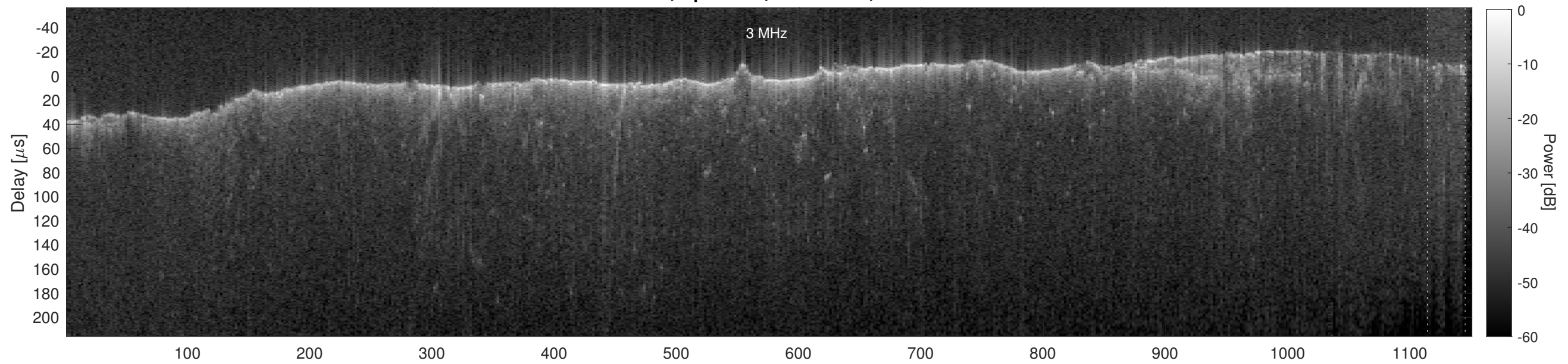
Orbit 11081, Cluttergram
