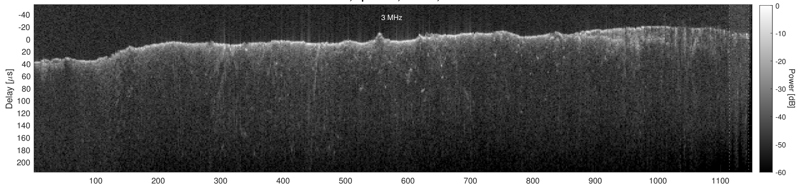
Orbit 11081, Cluttergram
