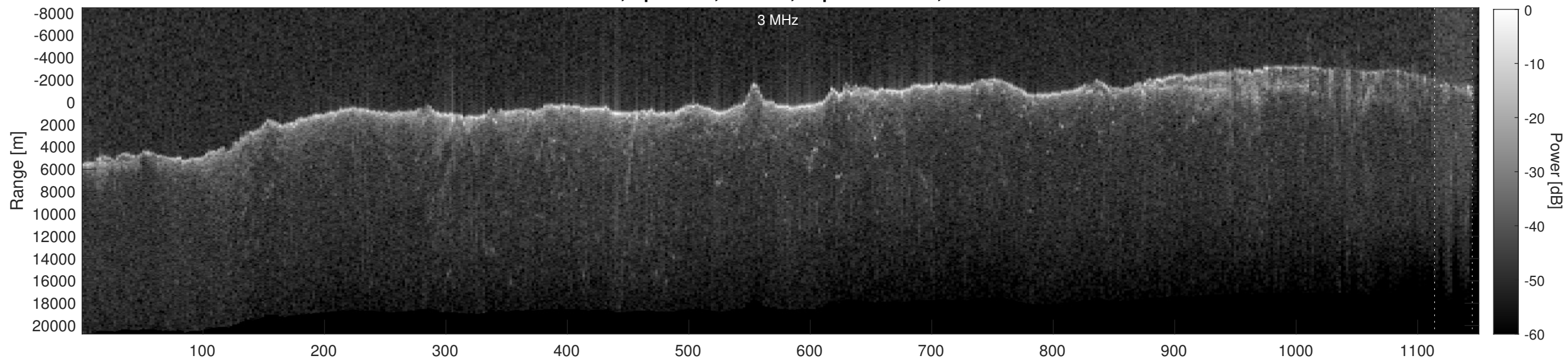
Orbit 11081, Depth-Corrected Cluttergram
