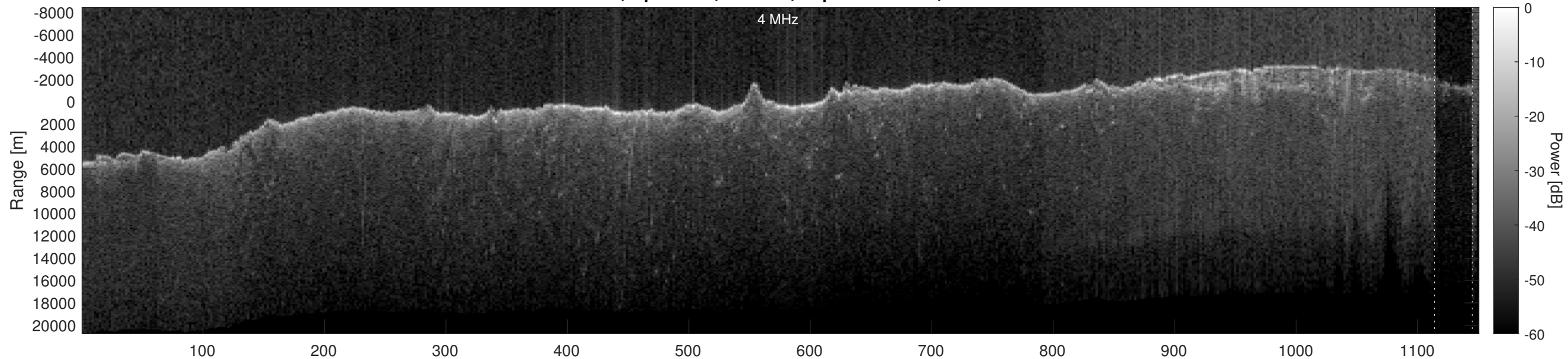
Orbit 11081, Optimized, Window, Depth-Corrected, Channel 2
