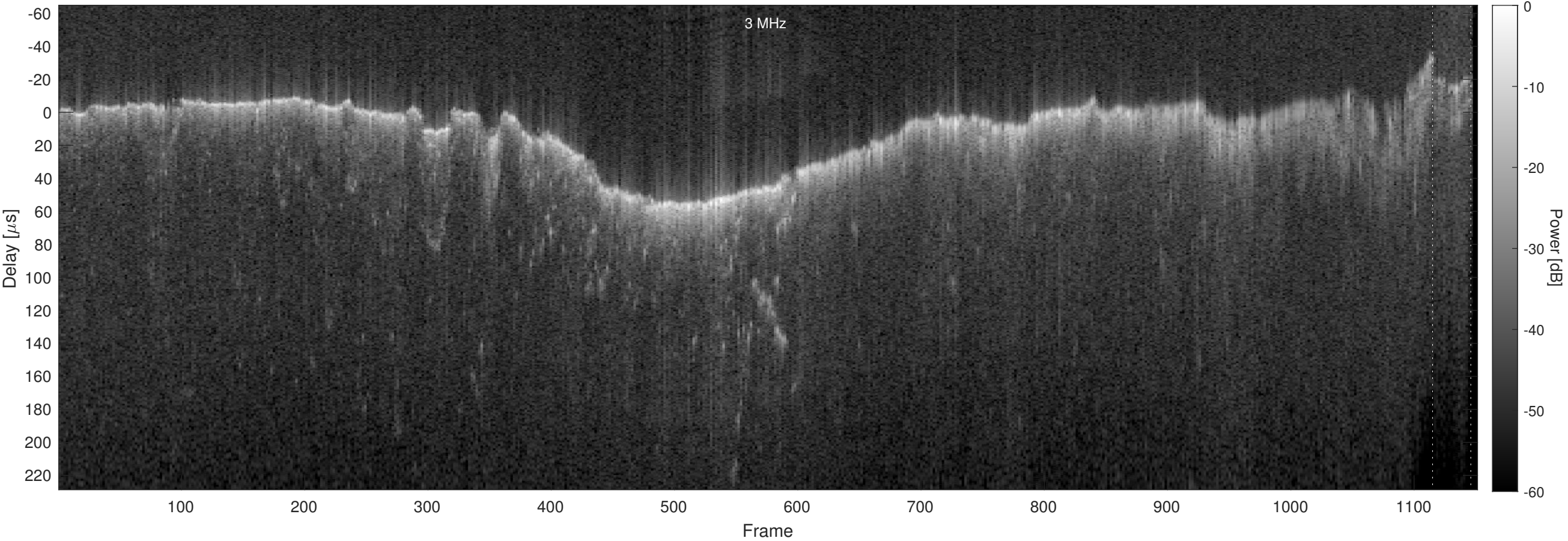
Orbit 11082, Chapman, No Window, Channel 2
