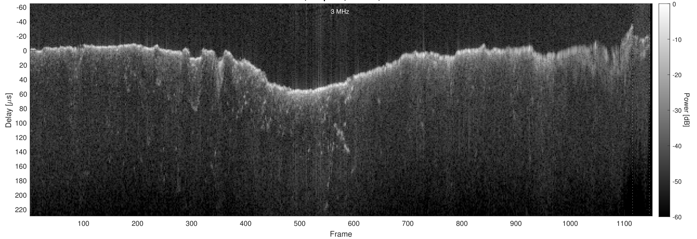
Orbit 11082, Chapman, Window, Channel 2
