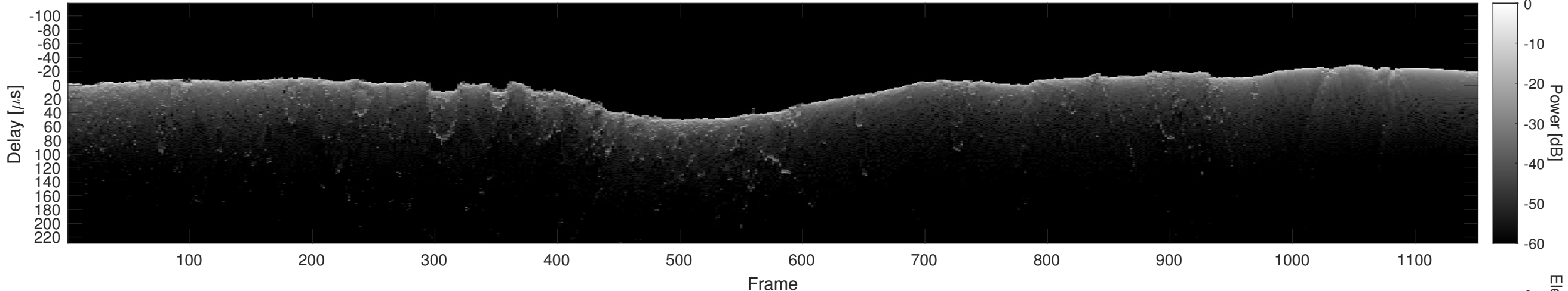
Orbit 11082, Cluttergram
