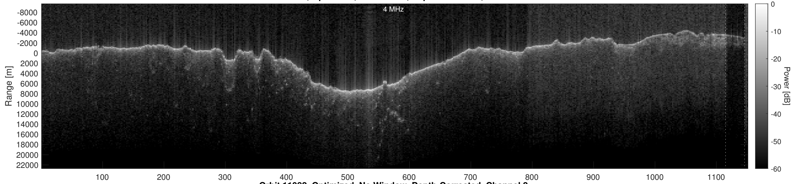
Orbit 11082, Optimized, No Window, Depth-Corrected, Channel 2
