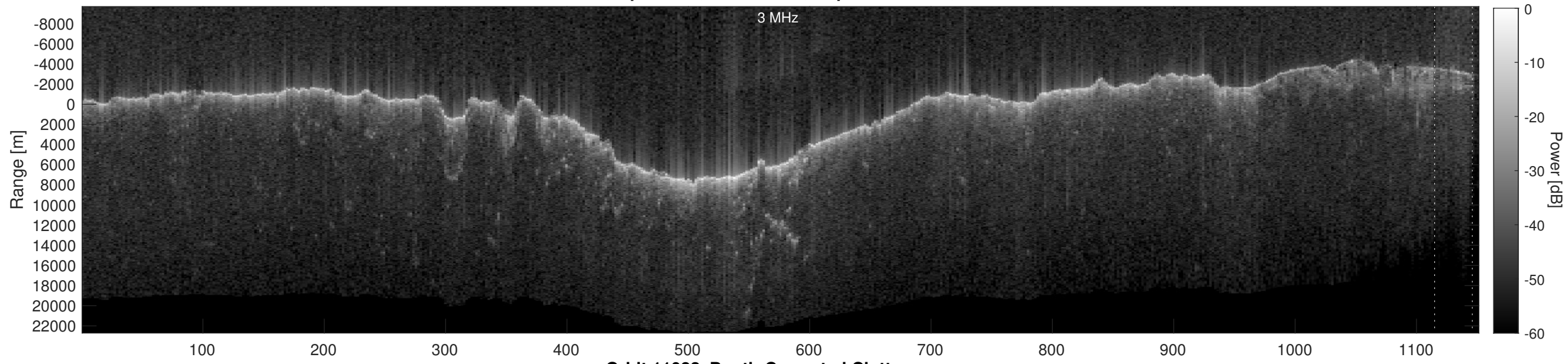
Orbit 11082, Depth-Corrected Cluttergram
