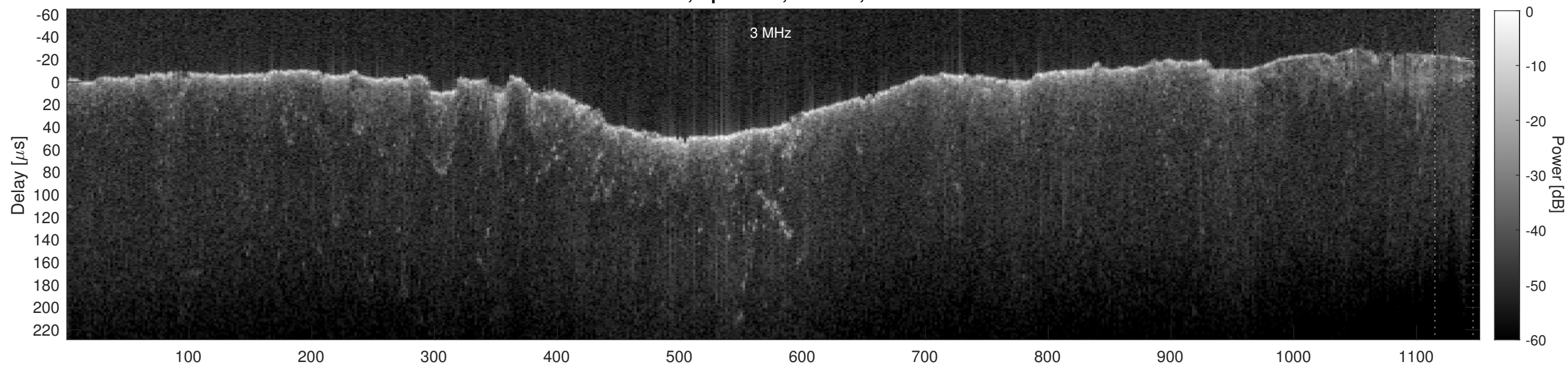
Orbit 11082, Cluttergram
