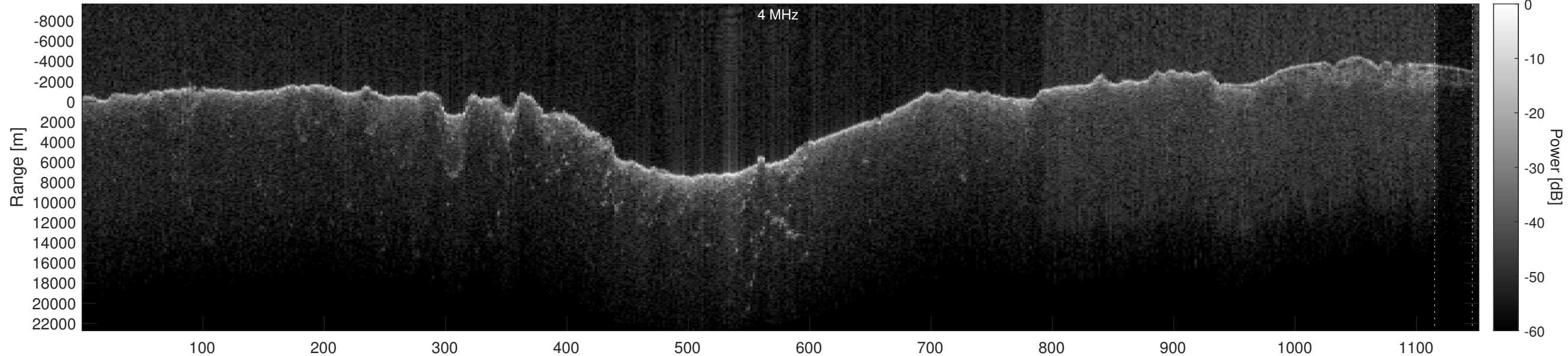
Orbit 11082, Optimized, Window, Depth-Corrected, Channel 2
