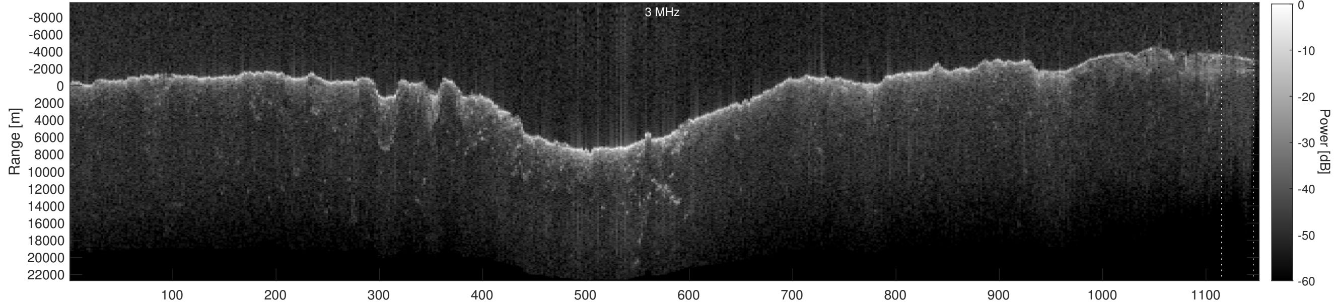
Orbit 11082, Depth-Corrected Cluttergram
