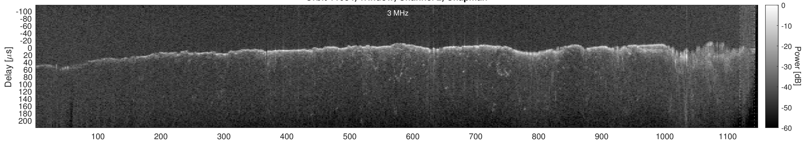
Orbit 11084, Window, Channel 2, Optimized
