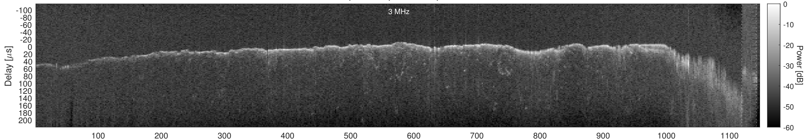
Orbit 11084, Window, Channel 2, Chapman
