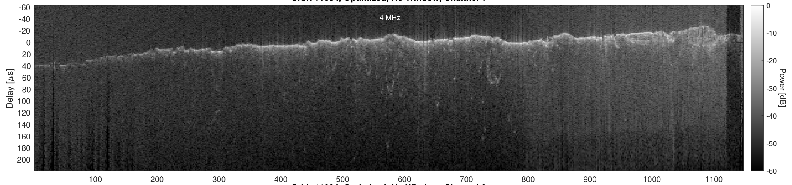
Orbit 11084, Optimized, No Window, Channel 2
