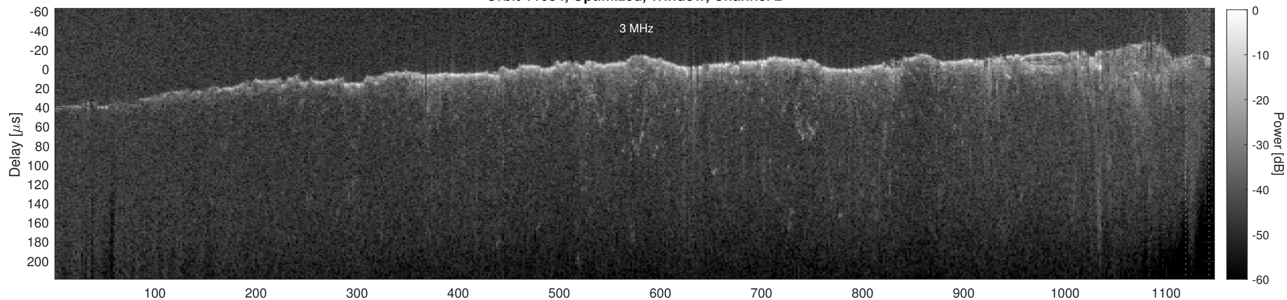
Orbit 11084, Cluttergram
