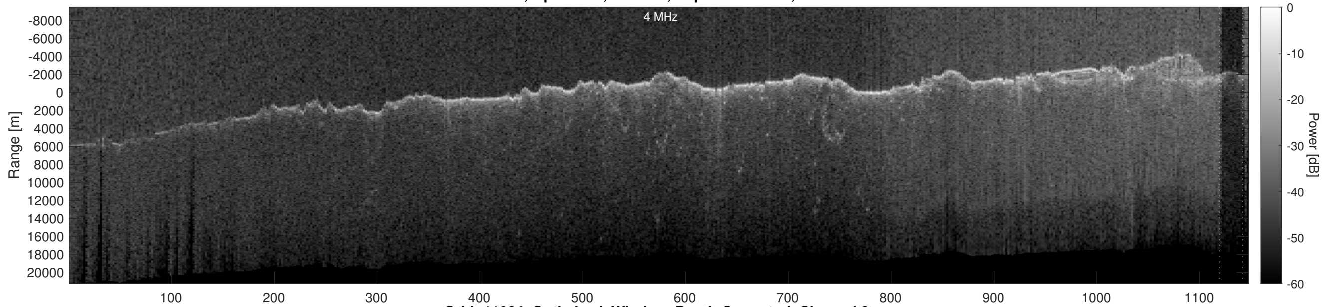
Orbit 11084, Optimized, Window, Depth-Corrected, Channel 2
