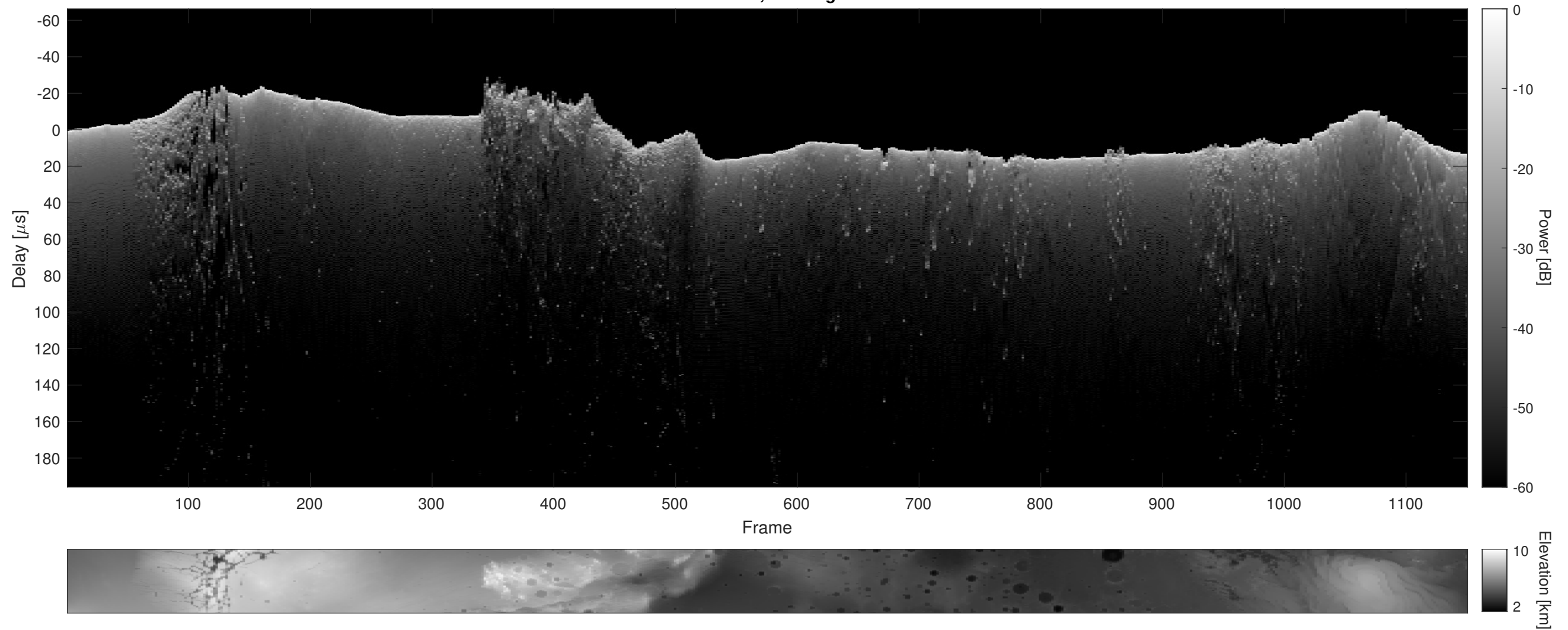
Orbit 11087, Cluttergram
