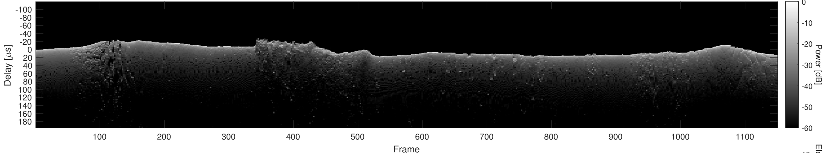
Orbit 11087, Cluttergram
