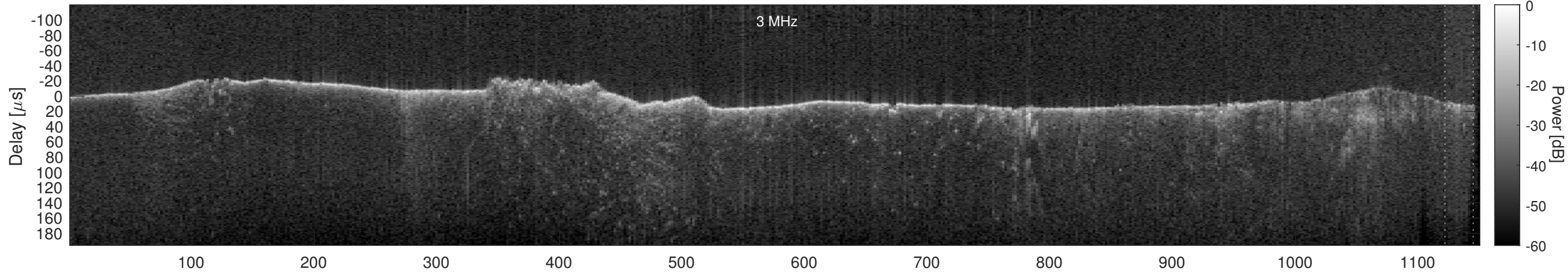
Orbit 11087, Cluttergram
