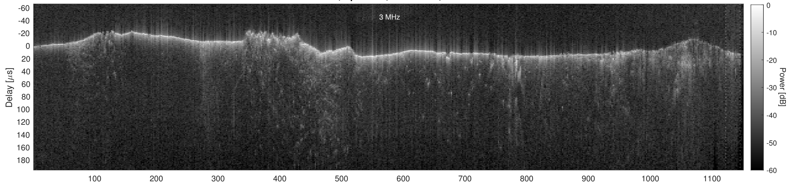
Orbit 11087, Cluttergram
