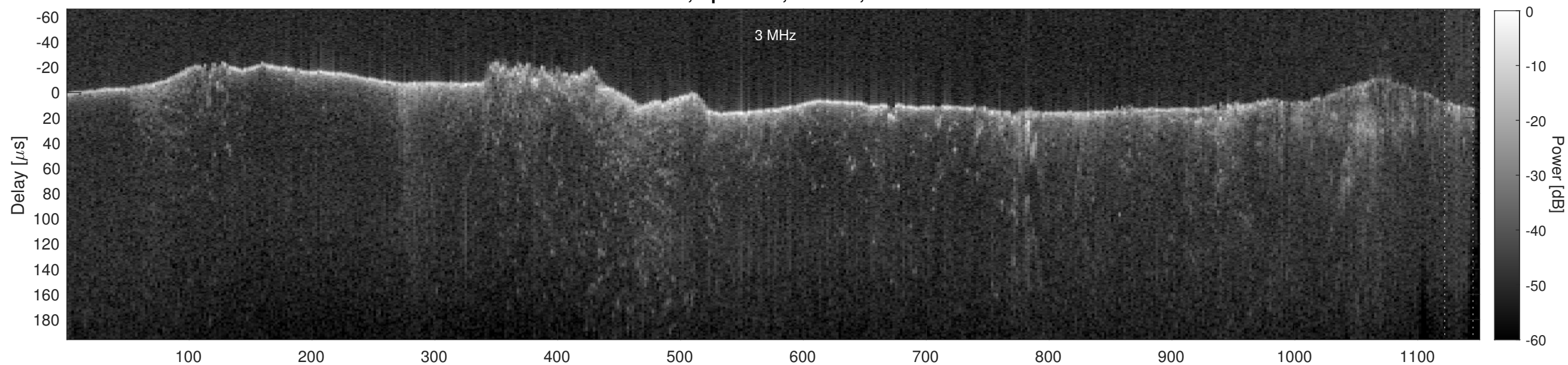
Orbit 11087, Cluttergram
