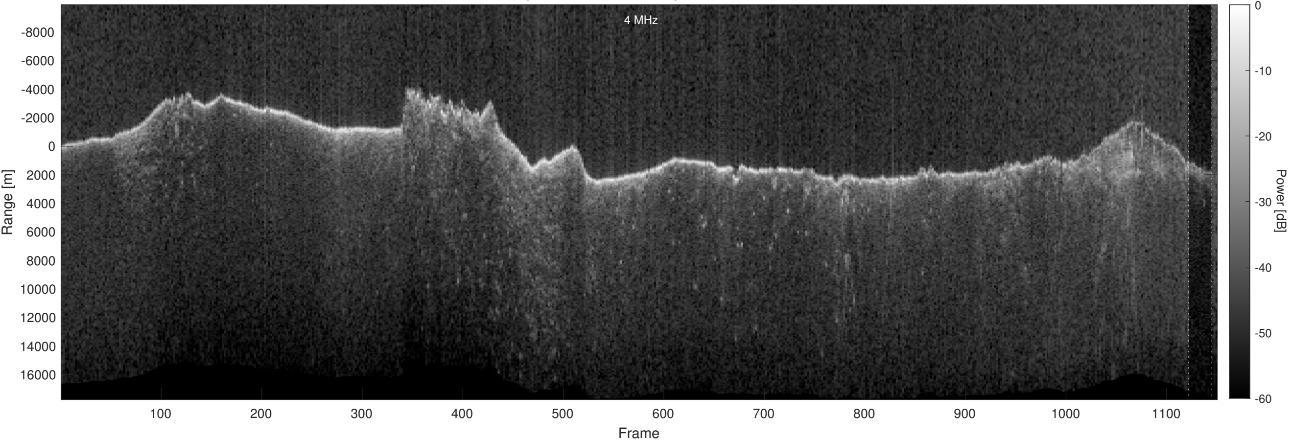
Orbit 11087, Optimized, Window, Depth-Corrected, Channel 2
